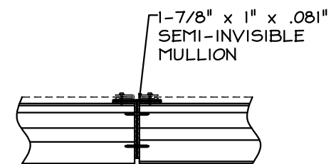
(EXTERIOR) SEMI-INVISIBLE MULLION
