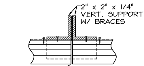
(EXTERIOR) VERTICAL INVISIBLE MULLION
