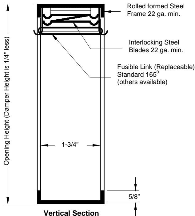
Vertical Section
