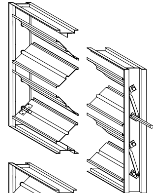
Model 610 Opposed Blade
