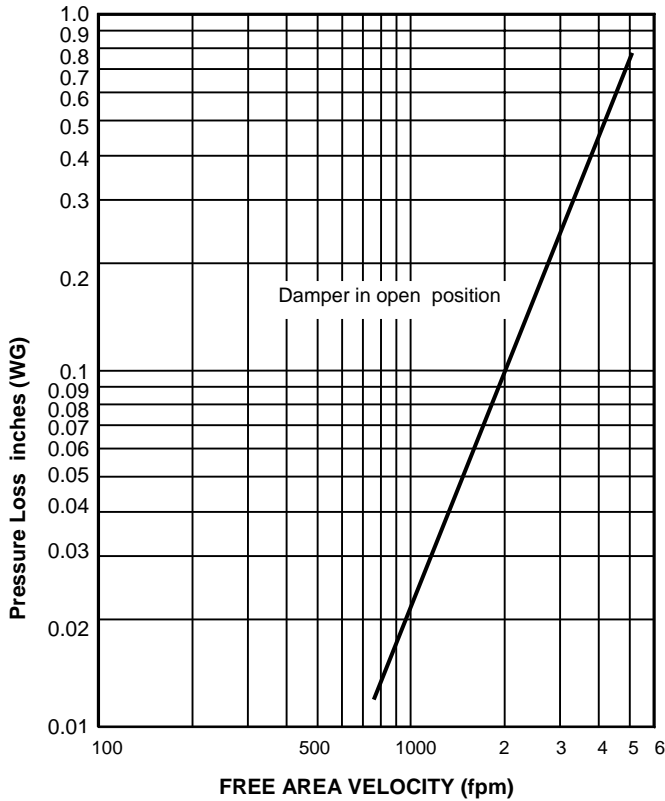
AIR PERFORMANCE
