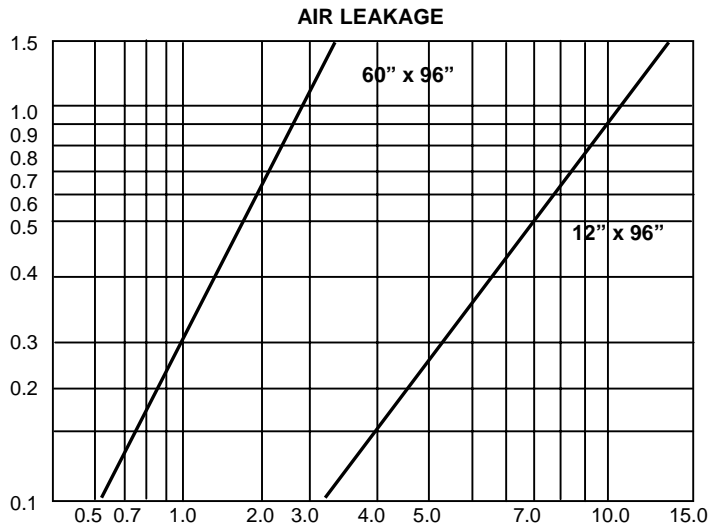
AIR LEAKAGE 60" x 96" 12" x 96" Air Leakage (cfm) Per Sq. Ft. of face area With blade and iamb seals
