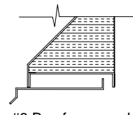
#8 Box frame and Sill Extension
