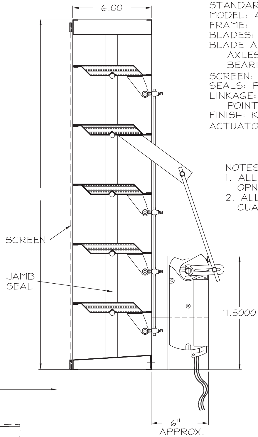
SECTION - "B"
