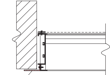
(C) FLANGE FRAME
