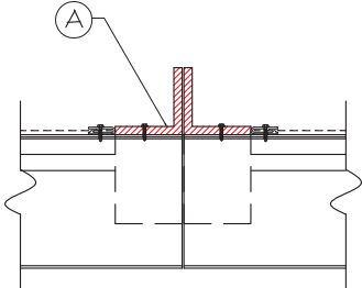
(A) VERTICAL INVISIBLE MULLION
