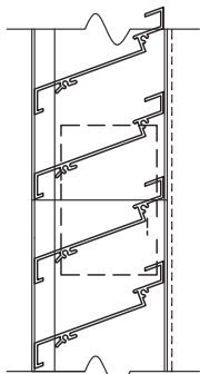
HORIZONTAL INVISIBLE MULLION
