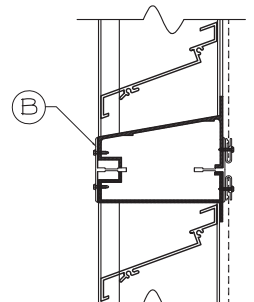
(B) HORIZONTAL VISIBLE MULLION
