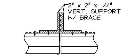
(EXTERIOR) VERTICAL INVISIBLE MULLION
