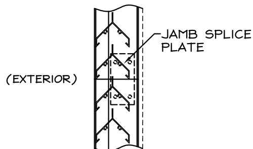
(EXTERIOR) HORIZONTAL INVISIBLE MULLION
