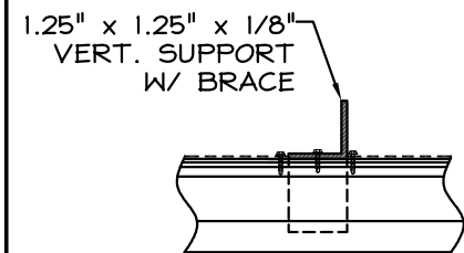
(EXTERIOR) CONTINUOUS BLADE
