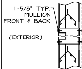
(EXTERIOR) HORIZONTAL VISIBLE MULLION
