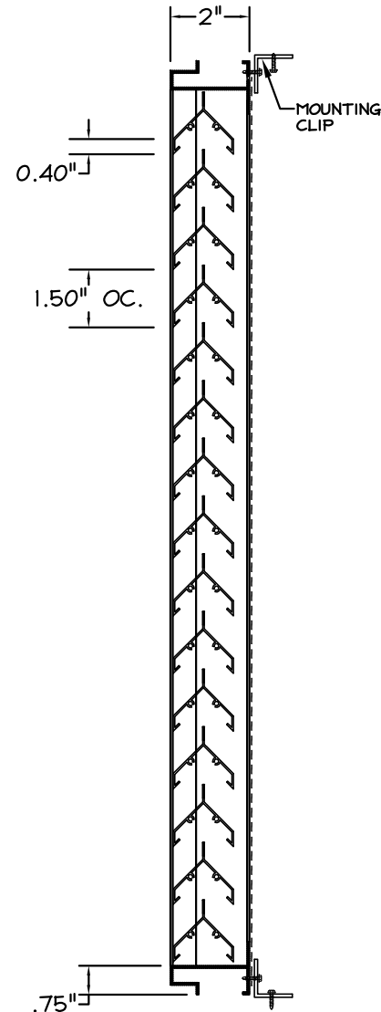
VERTICAL SECTION
