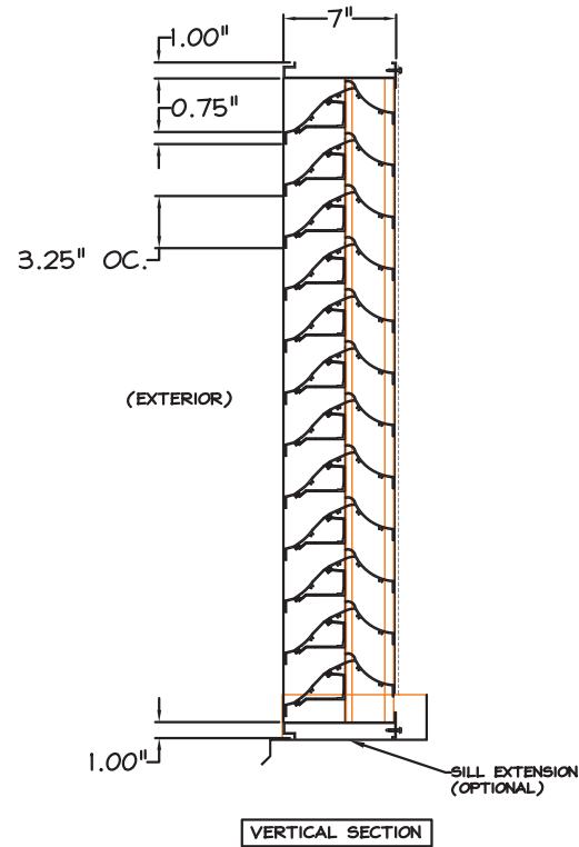
VERTICAL SECTION
