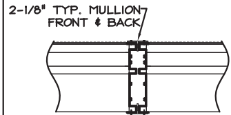
(EXTERIOR) VERTICAL VISIBLE MULLION
