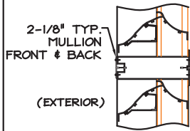
(EXTERIOR) HORIZONTAL VISIBLE MULLION
