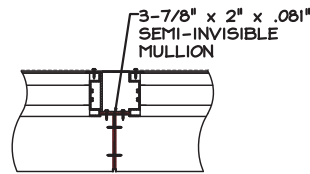
(EXTERIOR) SEMI-INVISIBLE MULLION
