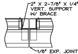
(EXTERIOR) VERTICAL INVISIBLE MULLION
