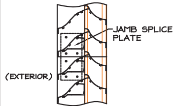
(EXTERIOR) HORIZONTAL INVISIBLE MULLION
