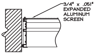
(EXTERIOR) BOX FRAME
