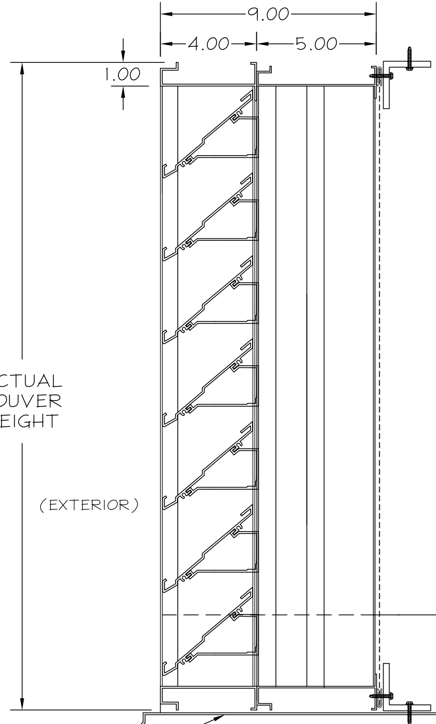
VERTICAL SECTION
