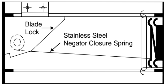
Horizontal Section
