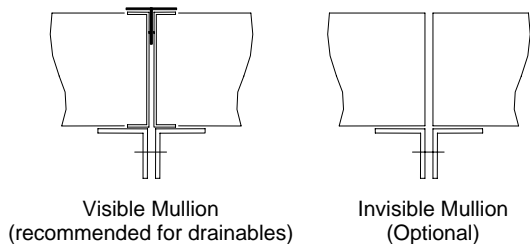
MULLION STYLE
